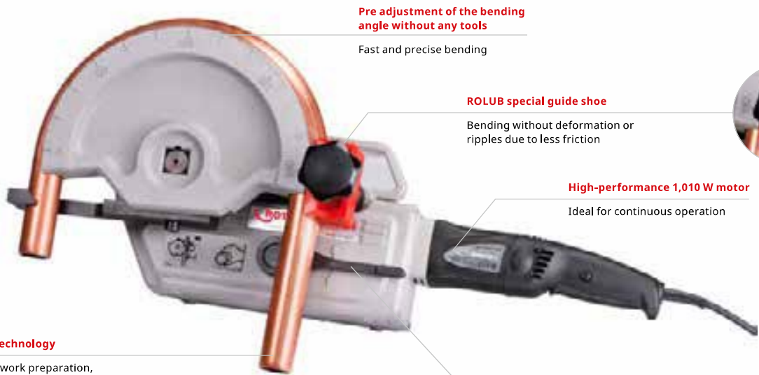
Automatic switch-off when preset bending angle is obtained Fast batch production possible
